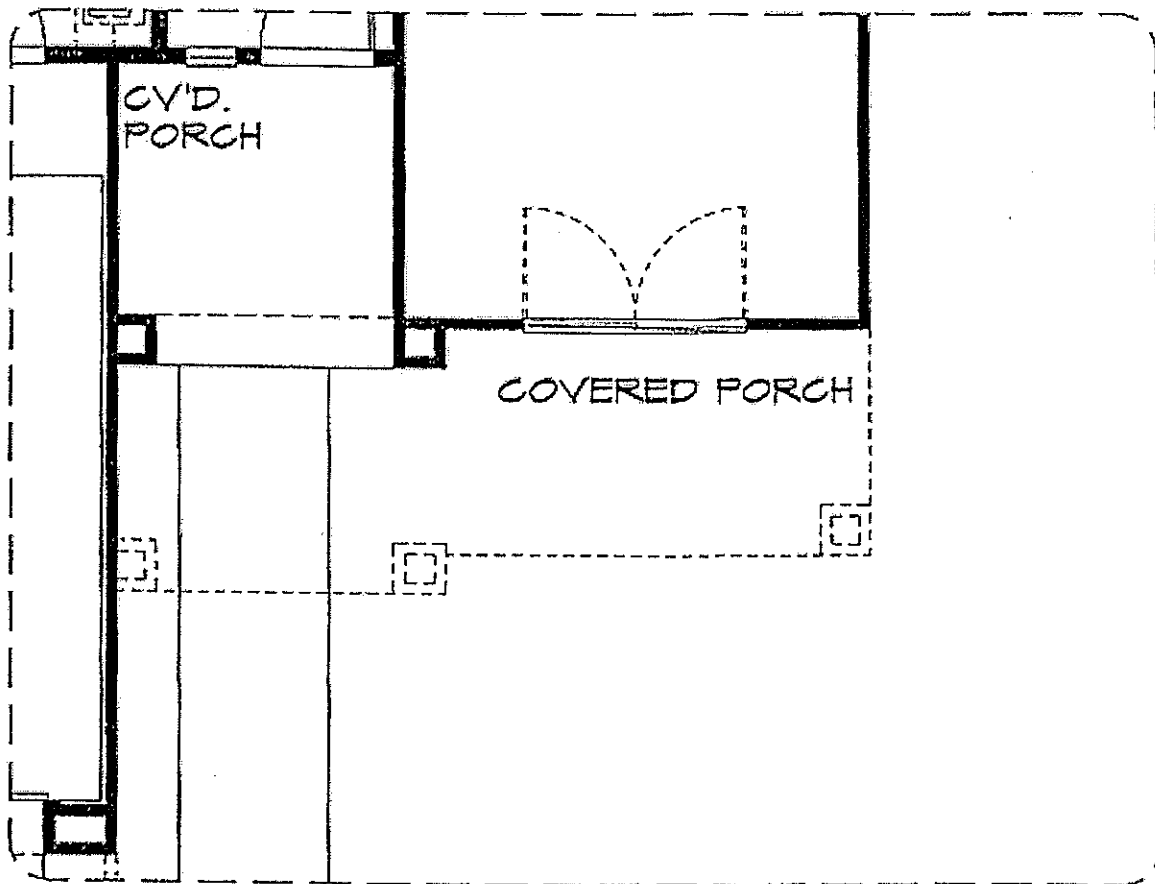
PARTIAL FLOOR PLAN - ELEV. B & D
