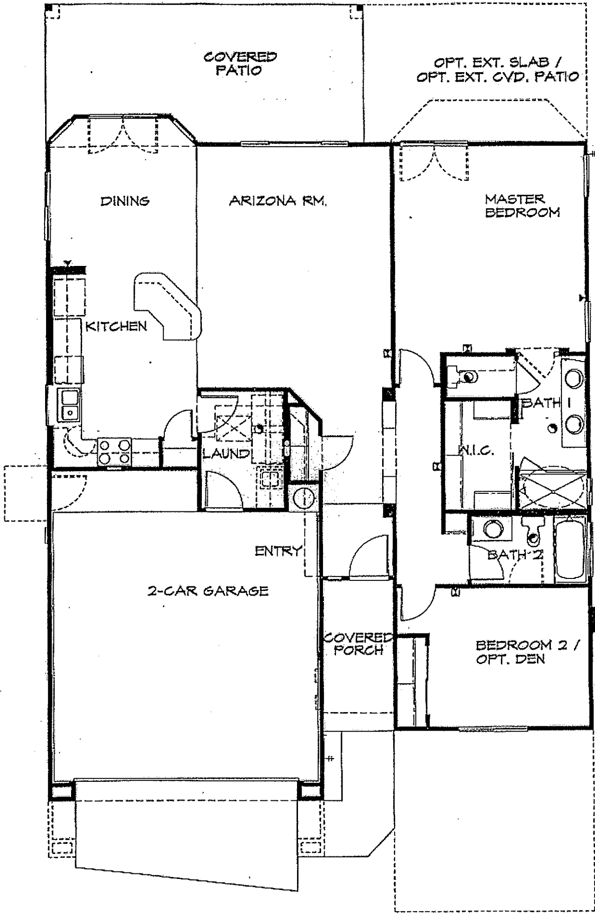
FLOOR PLAN - 9028
